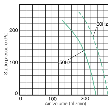
AF-60S-2-E AF-60S-2 AFS-60S-2-E AFS-60S-2 φ600mm 3-phase 1.5/2.2kW 4P 200V 50/60Hz
